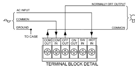
Diagram 4. SWITCHED LOADS
