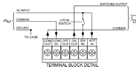
Diagram 4. SWITCHED LOADS
