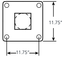
1" Base Plate
