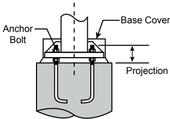
Base Detail
