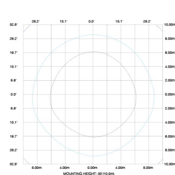
ISOLUX DIAGRAM
