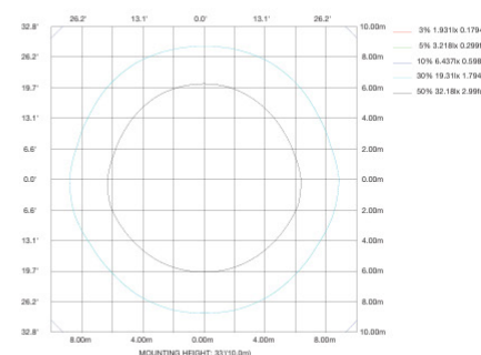
ISOLUX DIAGRAM
