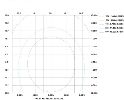
ISOLUX DIAGRAM
