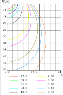
CO PLANE ISOLUX DIAGRAM (UNIT:lx)
