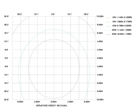
ISOLUX DIAGRAM
