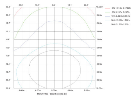
ISOLUX DIAGRAM
