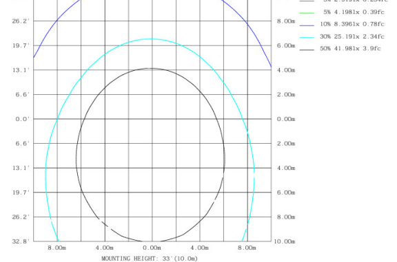
ISOLUX DIAGRAM
