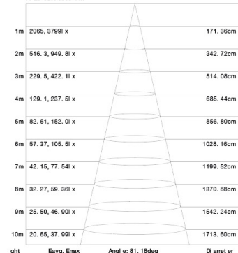
Flux out: 4903 lm
