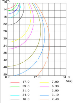
C0 PLANE ISOLUX DIAGRAM (UNIT:lx)
