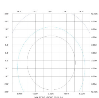
ISOLUX DIAGRAM
