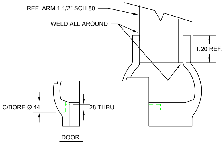
CROSS SECTION
