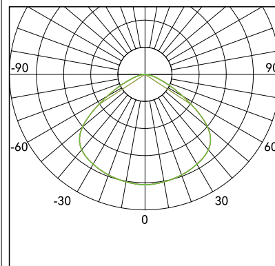
115 115° Beam Angle
