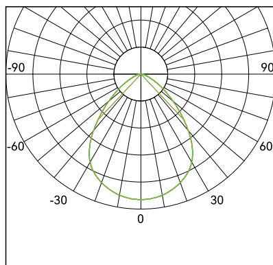
85 85° Beam Angle
