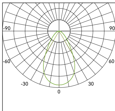
60 60° Beam Angle
