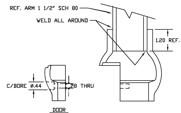
CROSS SECTION
