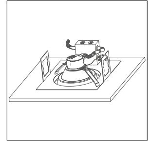
Ensure fixture is flush. Installation is complete
