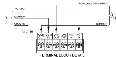
Diagram 4. SWITCHED LOADS
