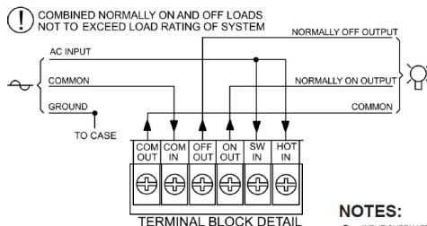
Diagram 3. NORMALLY ON & OFF LOADS
