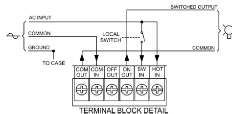
Diagram 4. SWITCHED LOADS
