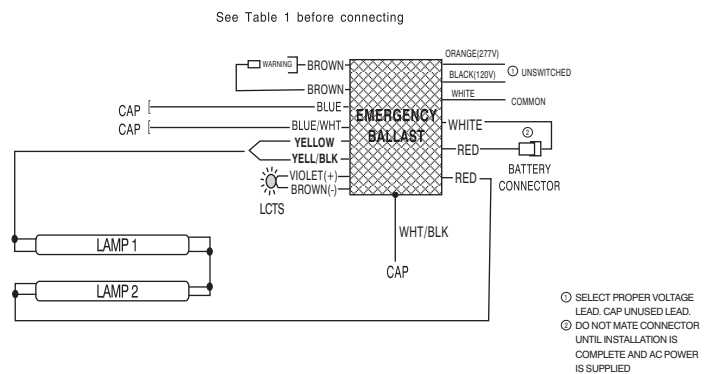
B. Two (2) Lamp Without AC Ballast
