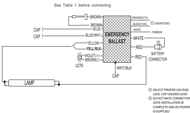
A. One (1) Lamp Without AC Ballast
